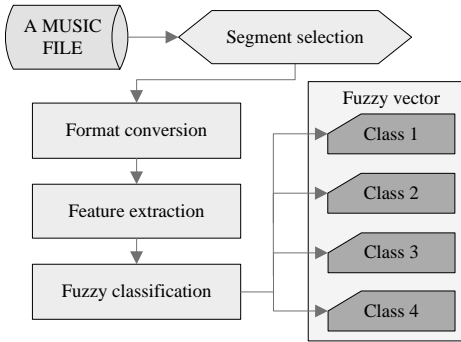
Figure 3. Block diagram of emotion classifier.
