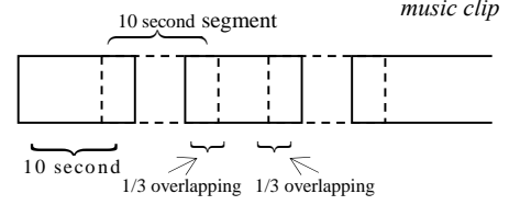
Figure 4. Segmentation of music clip in MEVD.
